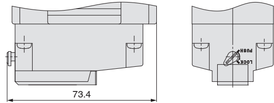
Details of manual override part (for manual operation)
