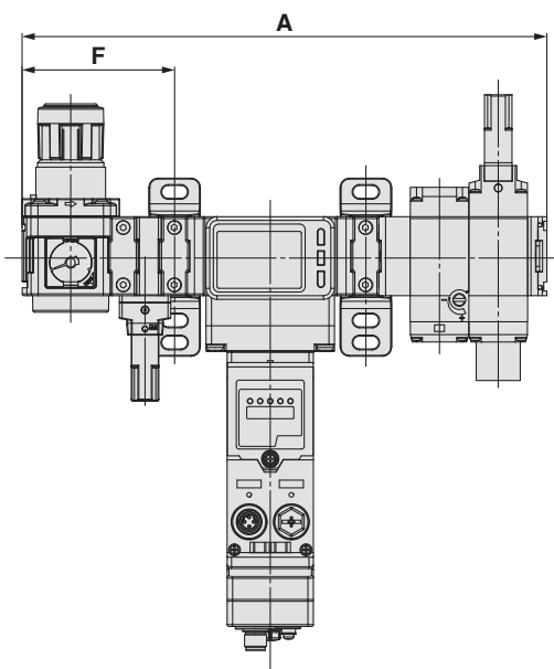
AMS20/30/40/60B-□00C (Without attachments)
