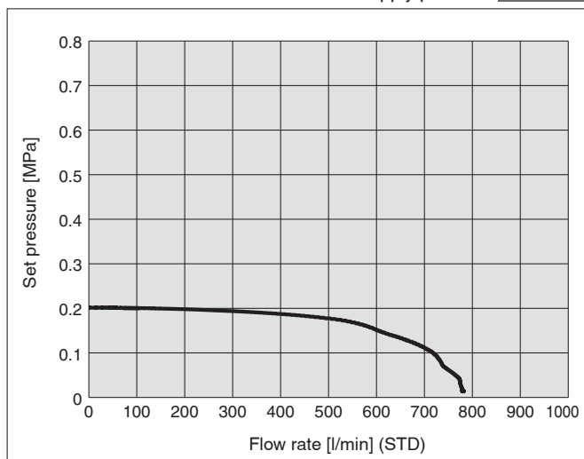
Supply pressure 0.3 MPa
