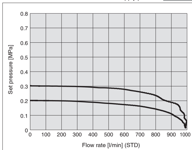
Supply pressure 0.4 MPa
