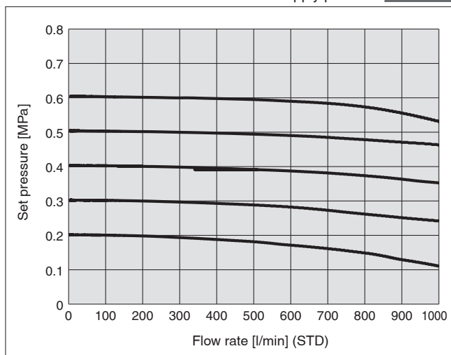
Supply pressure 0.7 MPa
