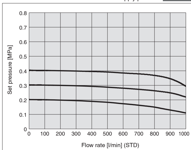
Supply pressure 0.5 MPa
