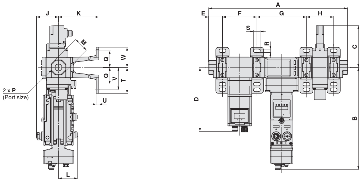
AMS20/30/40/60A-H00C (Without attachments)
