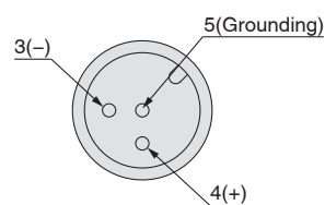
Detailed figure of a section M12 connector
