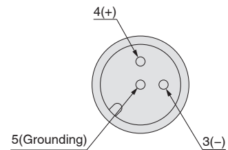
Detailed figure of b section M12 connector
