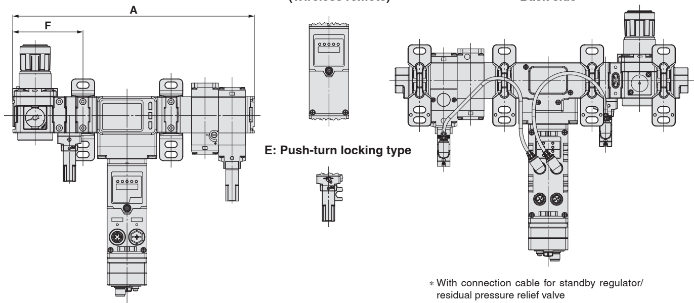
AMS20/30/40/60B-□00D (Without attachments)
