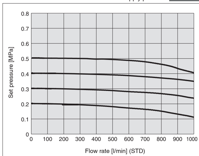
Supply pressure 0.6 MPa
