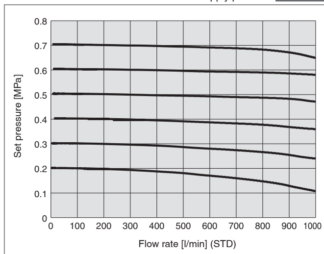
Supply pressure 0.8 MPa
