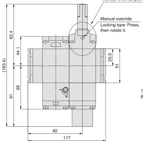
Manual override part
